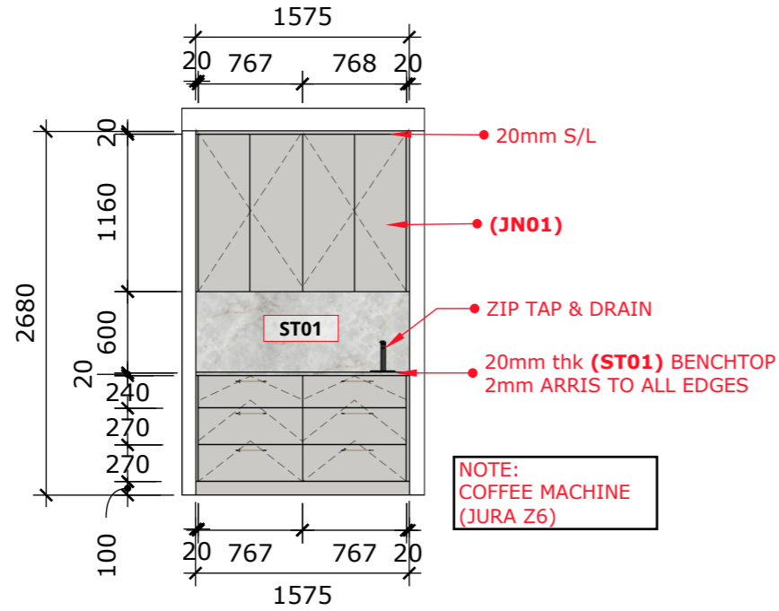
A :: KITCHEN ELEVATION 5 001 scale: 1=50mm
