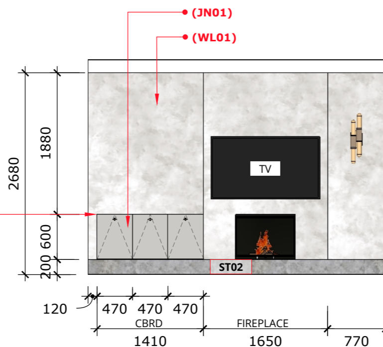
A :: FAMILY AREA FRONT ELEV. 003 scale: 1=50mm
