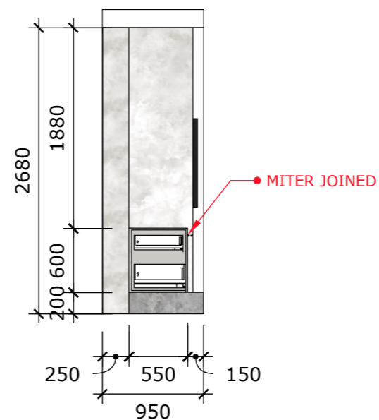
A :: FAMILY AREA SECTION 002 scale: 1=50mm
