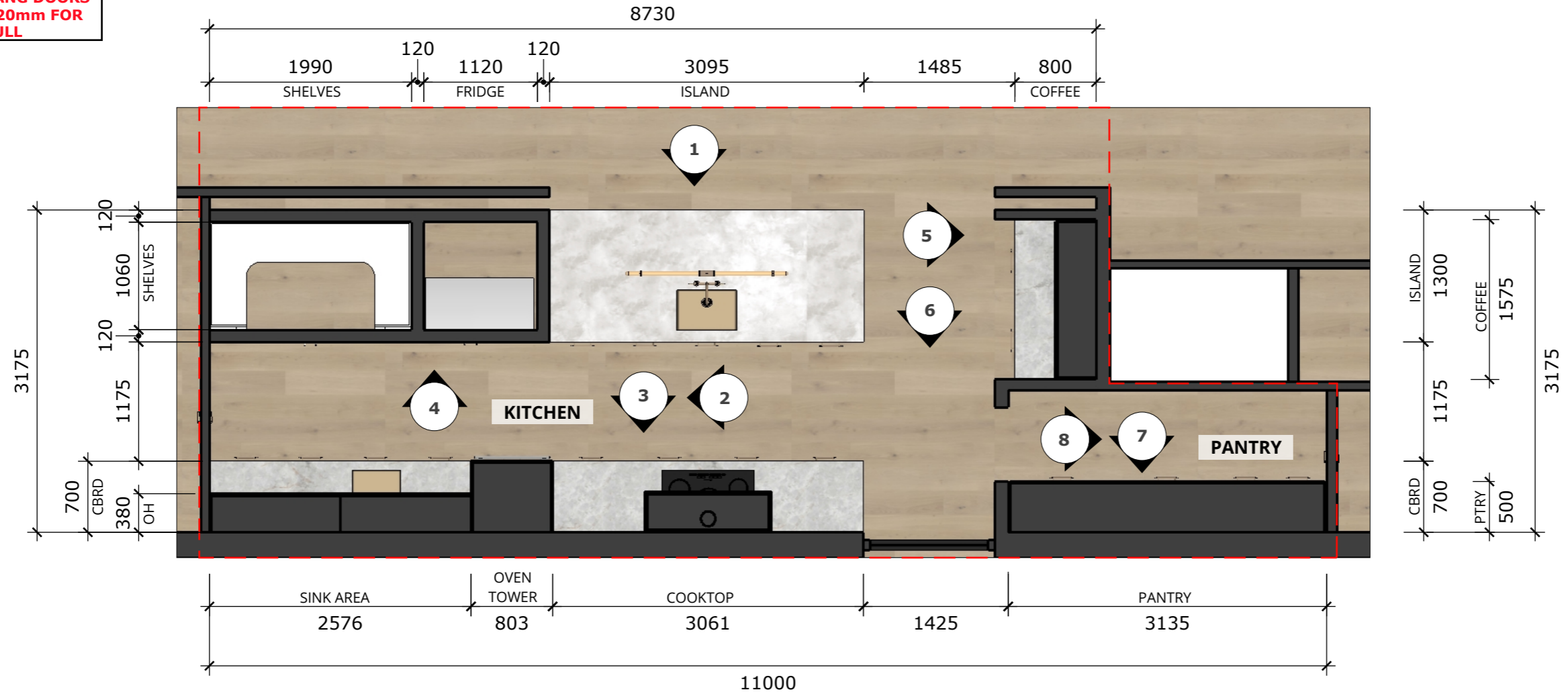
A :: KITCHEN PLAN 001 scale: 1=50mm
