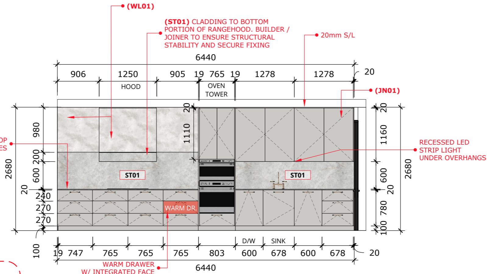
A :: KITCHEN ELEVATION 3 001 scale: 1=50mm
