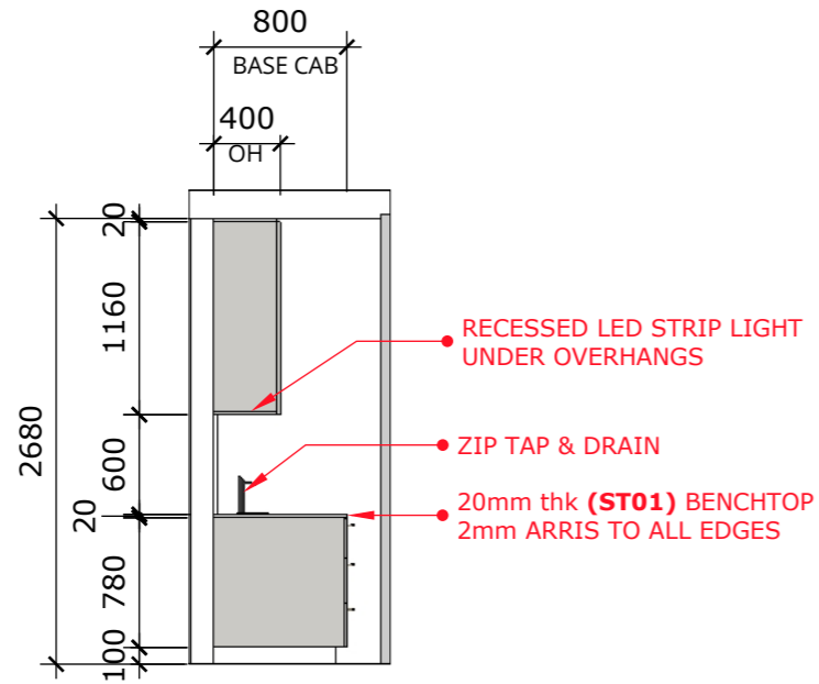
A :: KITCHEN ELEVATION 6 002 scale: 1=50mm
