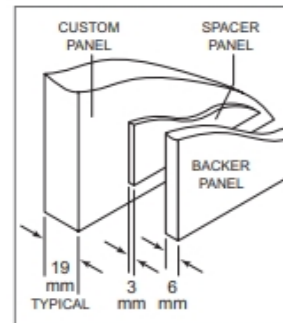
Panel assembly (rear view)
