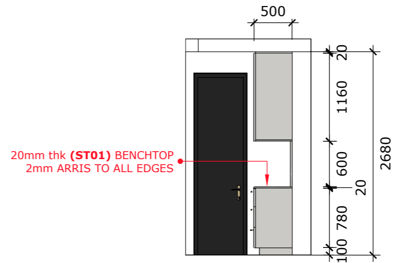
A :: KITCHEN ELEVATION 8 004 scale: 1=50mm
