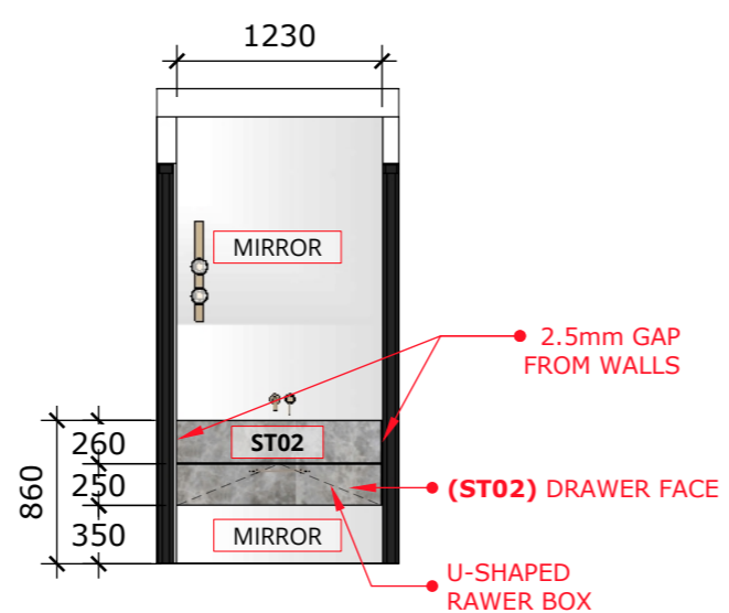
A :: VANITY FRONT ELEV 001 scale: 1=50mm
