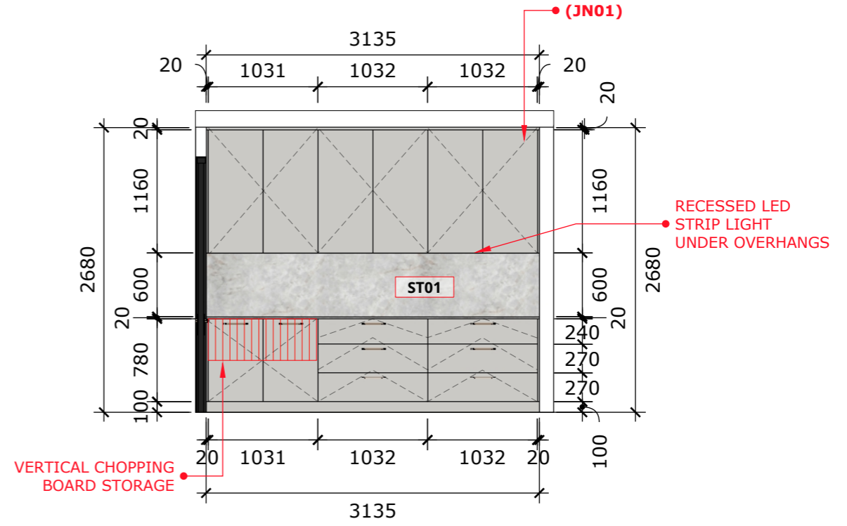
A :: KITCHEN ELEVATION 7 003 scale: 1=50mm
