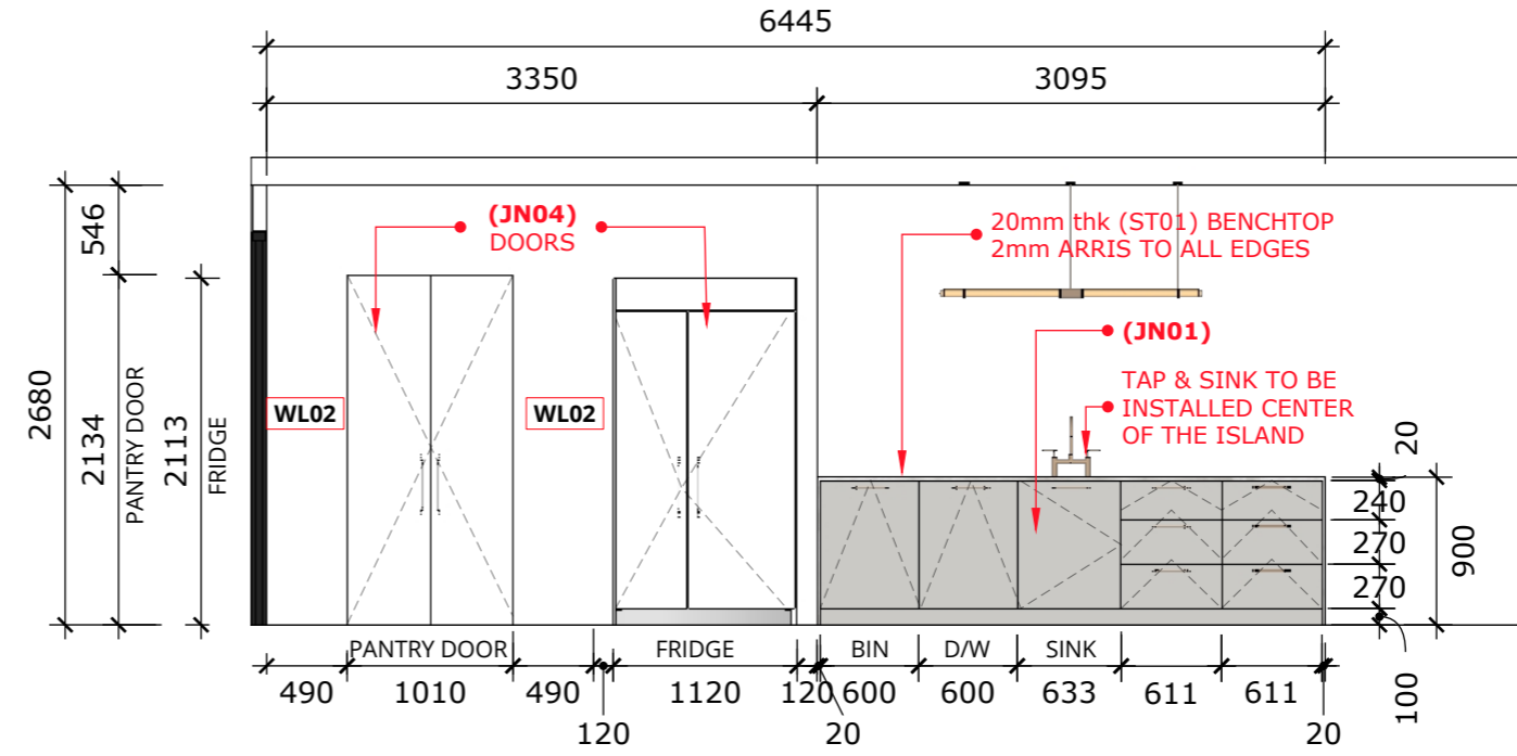
A :: KITCHEN ELEVATION 4 002 scale: 1=50mm
