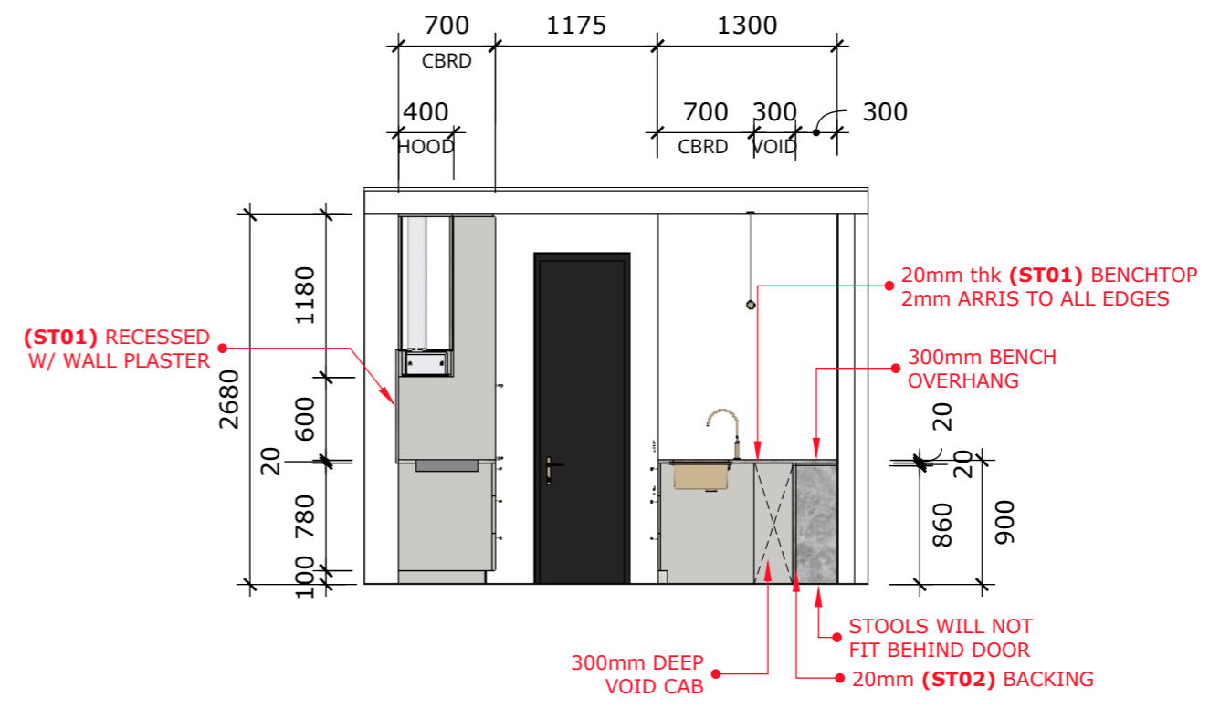
A :: KITCHEN ELEVATION 2 003 scale: 1=50mm
