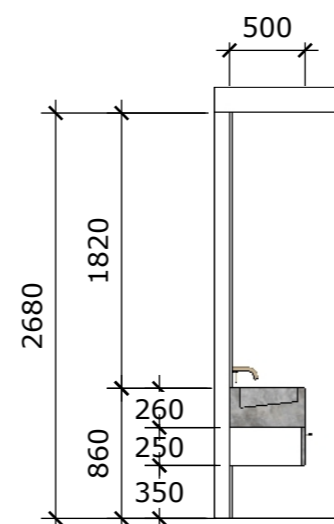
A :: VANITY SECTION 002 scale: 1=50mm
